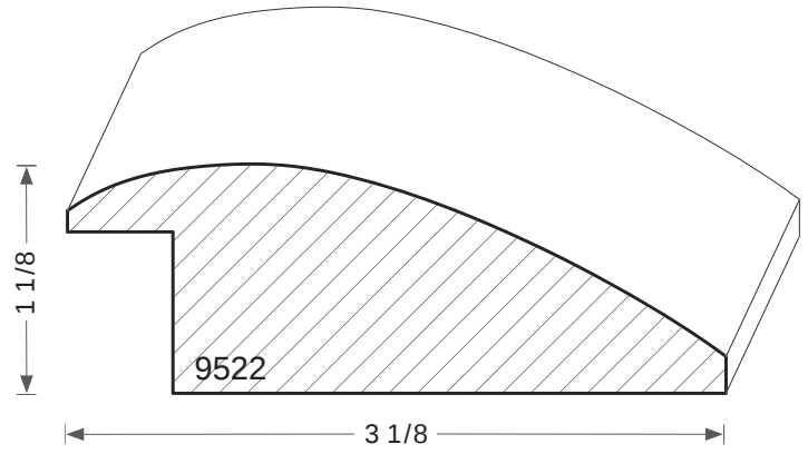
RABBET 7/8 X 1/2
