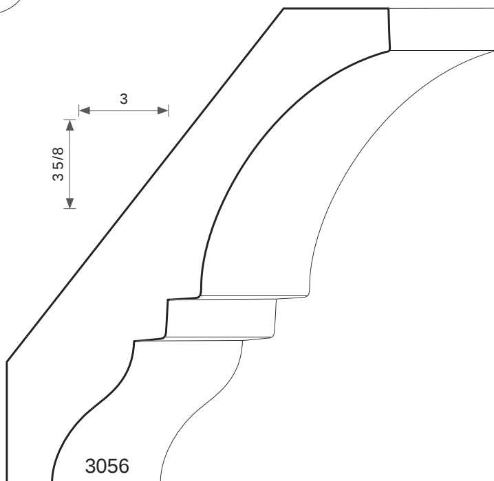
13/16T X 4-9/16W
