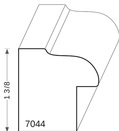
7044 RABBET 3/8 X 3/4
