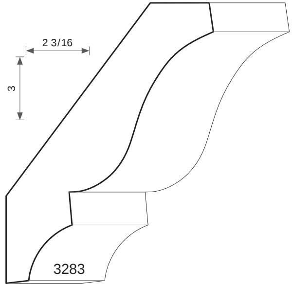
3/4T X 3-5/8W
