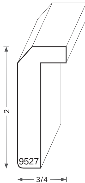
RABBET 1 3/4 X 3/8
