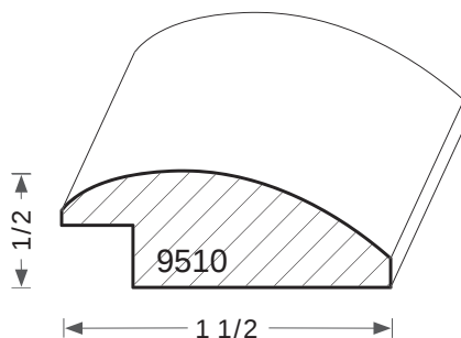
RABBET 1/4H X 1/4W
