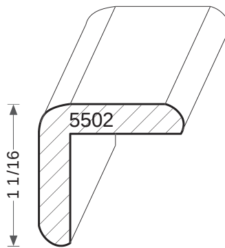
RABBET 7/8 X 7/8
