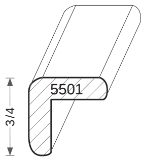
RABBET 9/16 X 9/16
