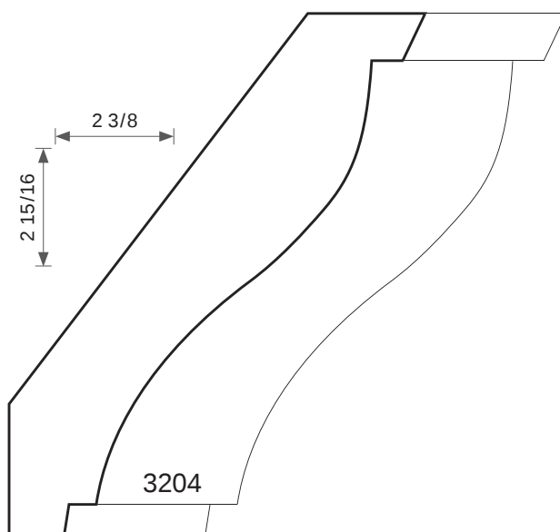
3/4T X 3-7/8W
