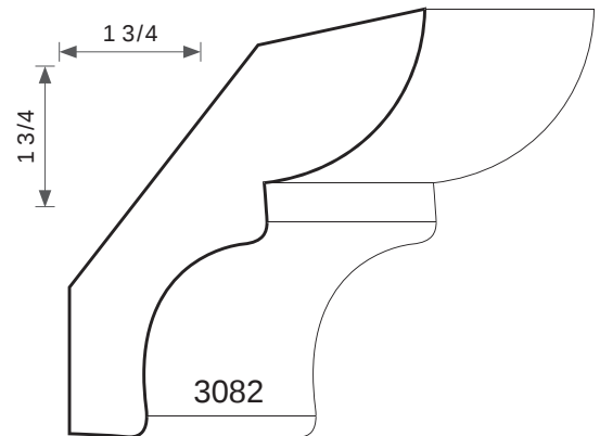
3/4T X 2-5/8W
