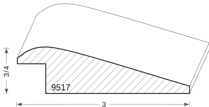
RABBET 1/2 X 1/2
