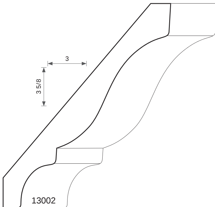
13002 9/16T X 4-5/8W
