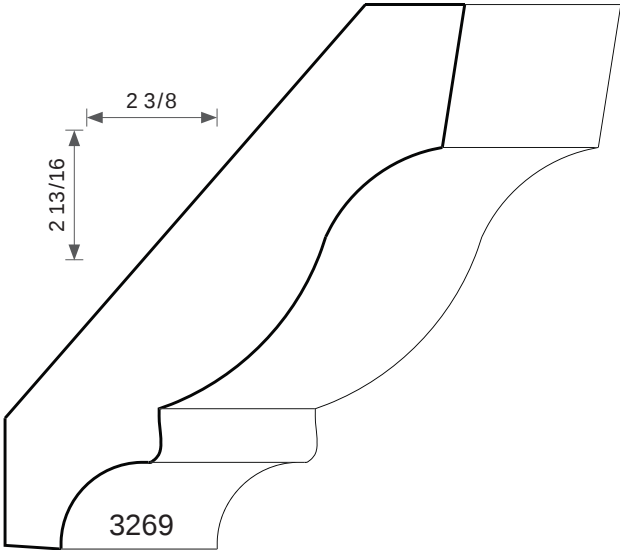
3/4T X 3-5/8W
