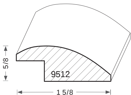
RABBET 3/8 X 1/2
