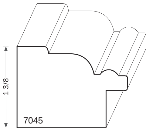
7045 RABBET 3/8 X 5/18
