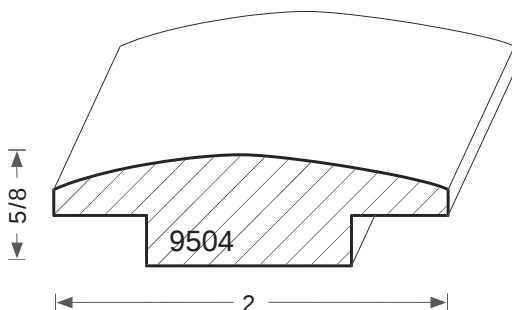
RABBET 1/4H X 1/2W
