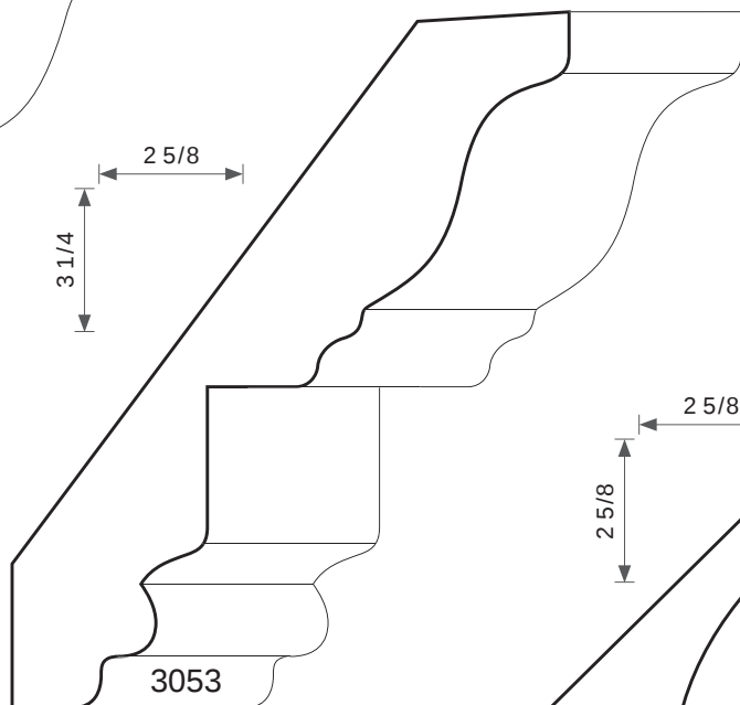
3/4T X 4-1/8W
