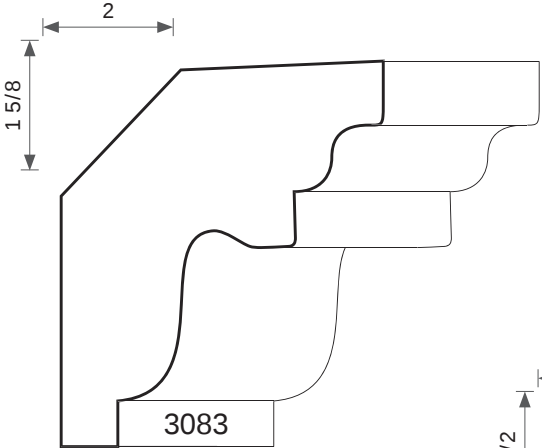
1-1/4T X 2-5/8W
