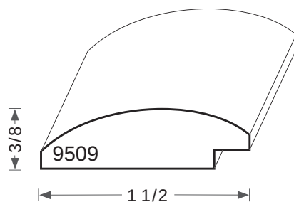
RABBET 1/8H X 1/4W
