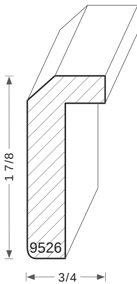
RABBET 1 5/8 X 3/8
