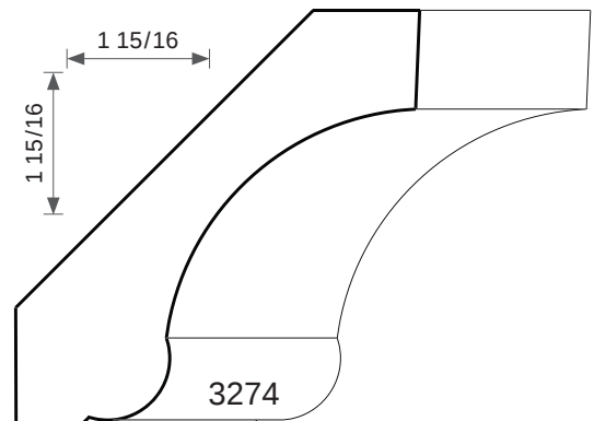
3/4T X 2-3/4W
