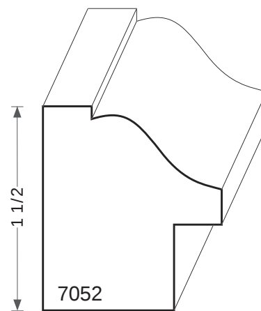
7052 RABBET 3/8 X 5/8
