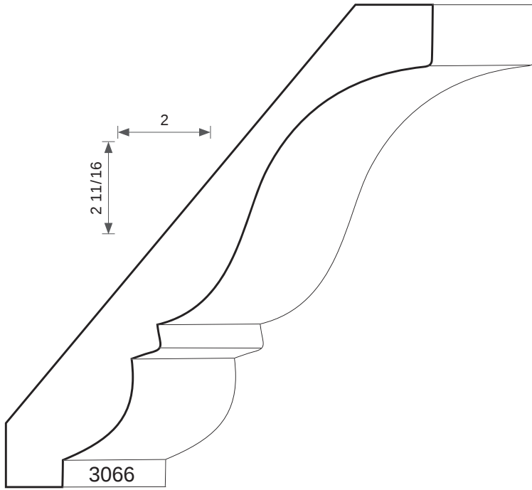
3/4T X 4-11/16W
