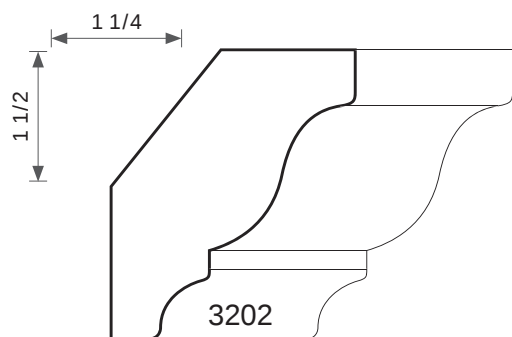
3/4T X 2W
