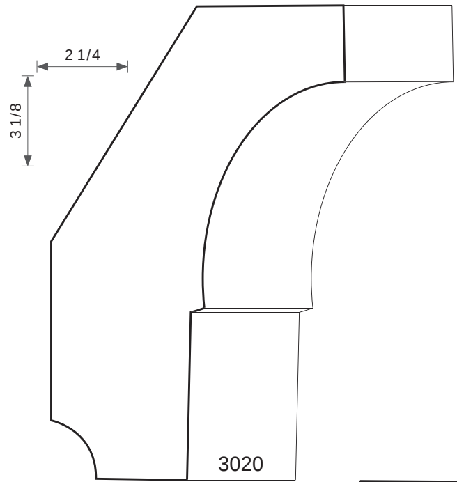
2-1/4T X 3-9/16W
