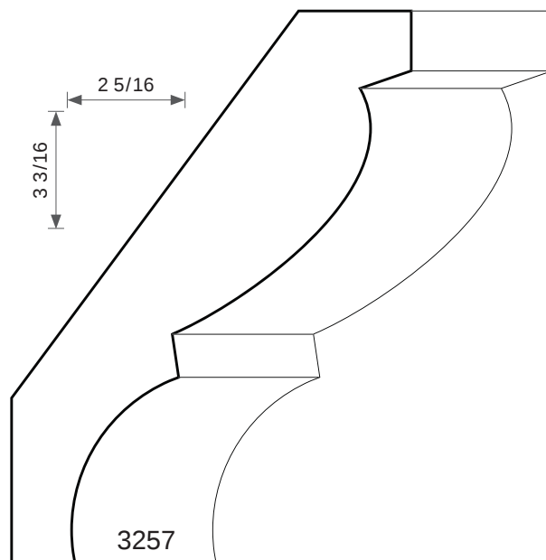
13/16T X 3-3/4W
