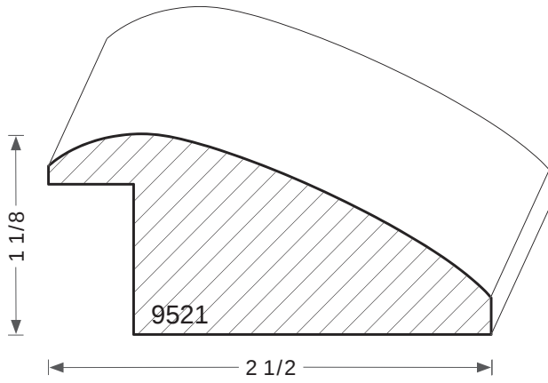
RABBET 7/8 X 1/2
