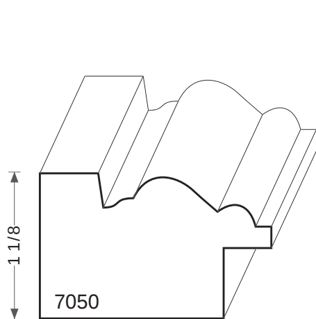
7050 RABBET 3/8 X 1/2
