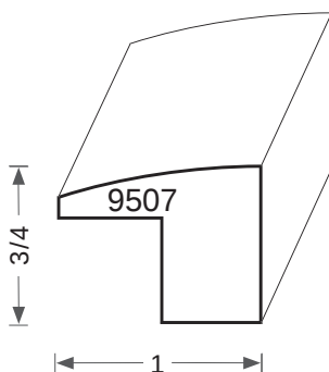
RABBET 1/2H X 1/2W
