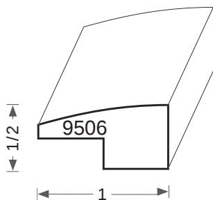
RABBET 1/4H X 1/2W
