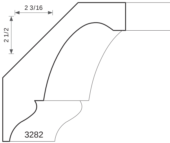
7/8T X 3-1/4W
