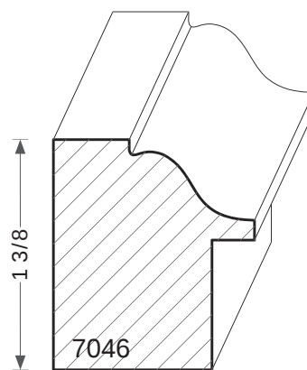
RABBET 1/4 X 3/4
