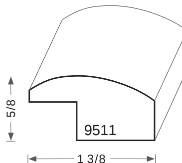
RABBET 3/8H X 1/2W
