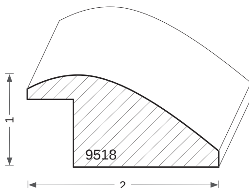
RABBET 3/4 X 1/2
