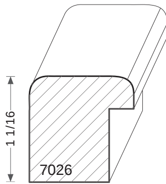
RABBET 1/4 X 3/4
