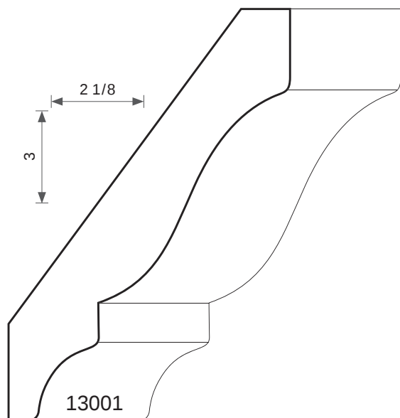
13001 9/16T X 3-5/8W
