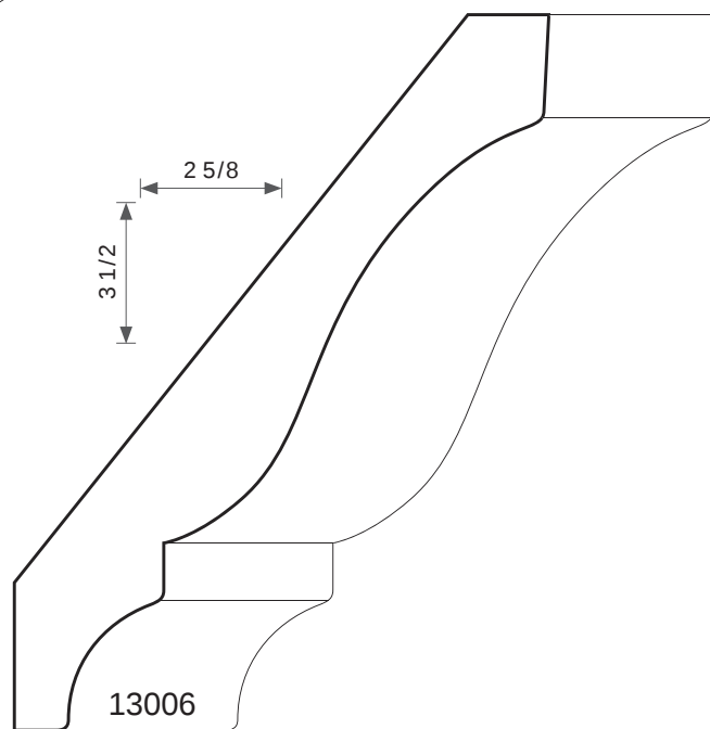
13006 5/8T X 4-1/4W
