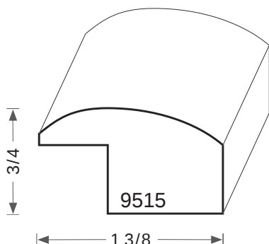
RABBET 1/2 X 1/2
