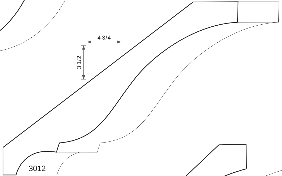
13/16T X 5-3/4W
