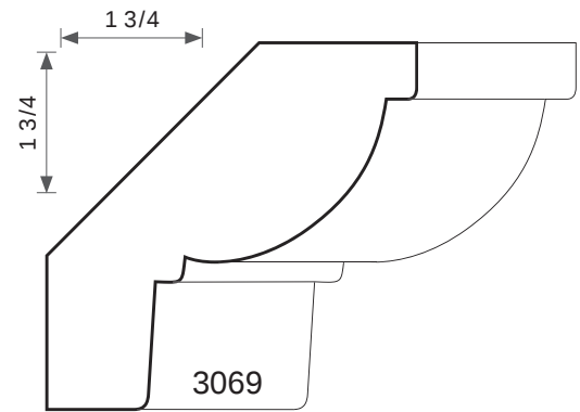
3/4T X 2-1/2W
