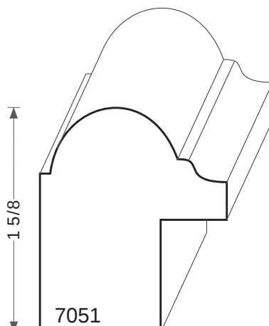
7051 RABBET 1/2 X 13/16
