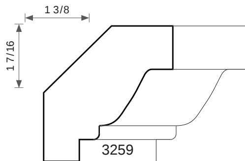
3/4T X 1-7/8W
