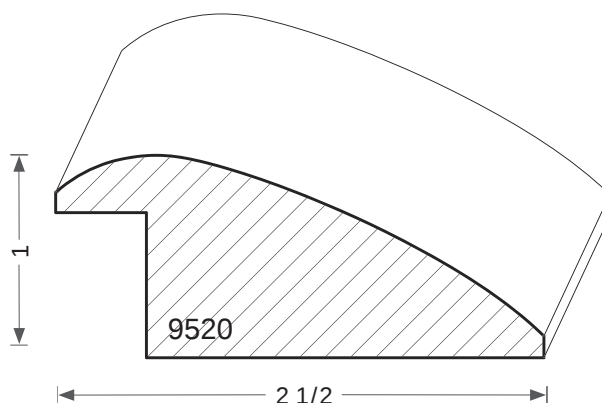
RABBET 3/4 X 1/2
