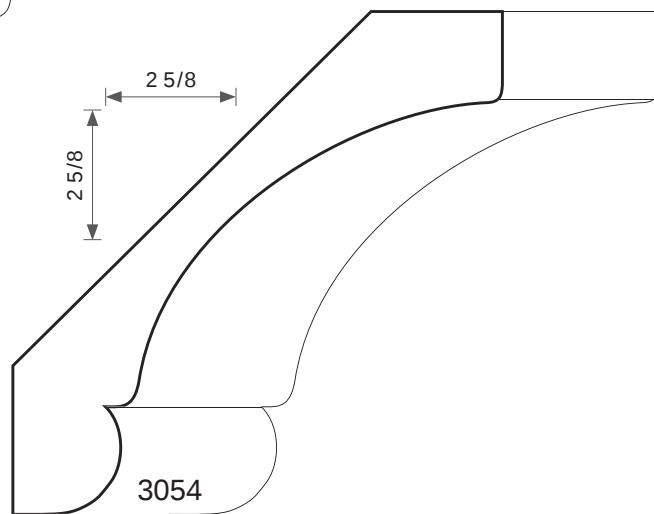
3/4T X 3-5/8W
