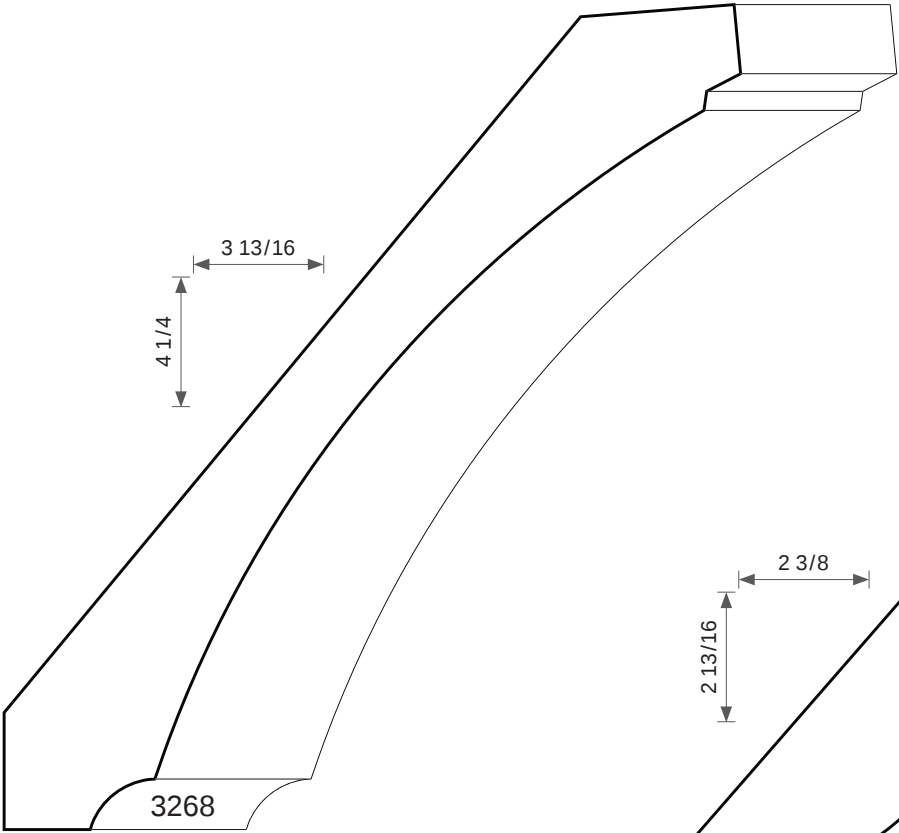
3/4T X 5-9/16W
