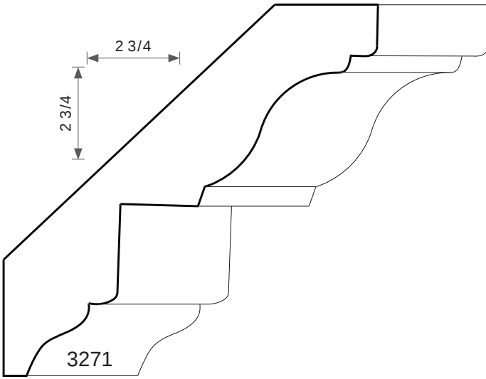
3/4T X 3-7/8W
