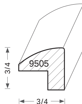
RABBET 1/4H X 1/2W
