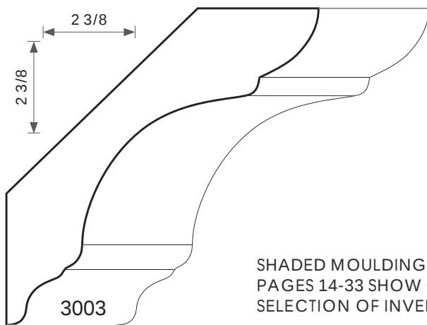
3/4T X 3-1/4W
