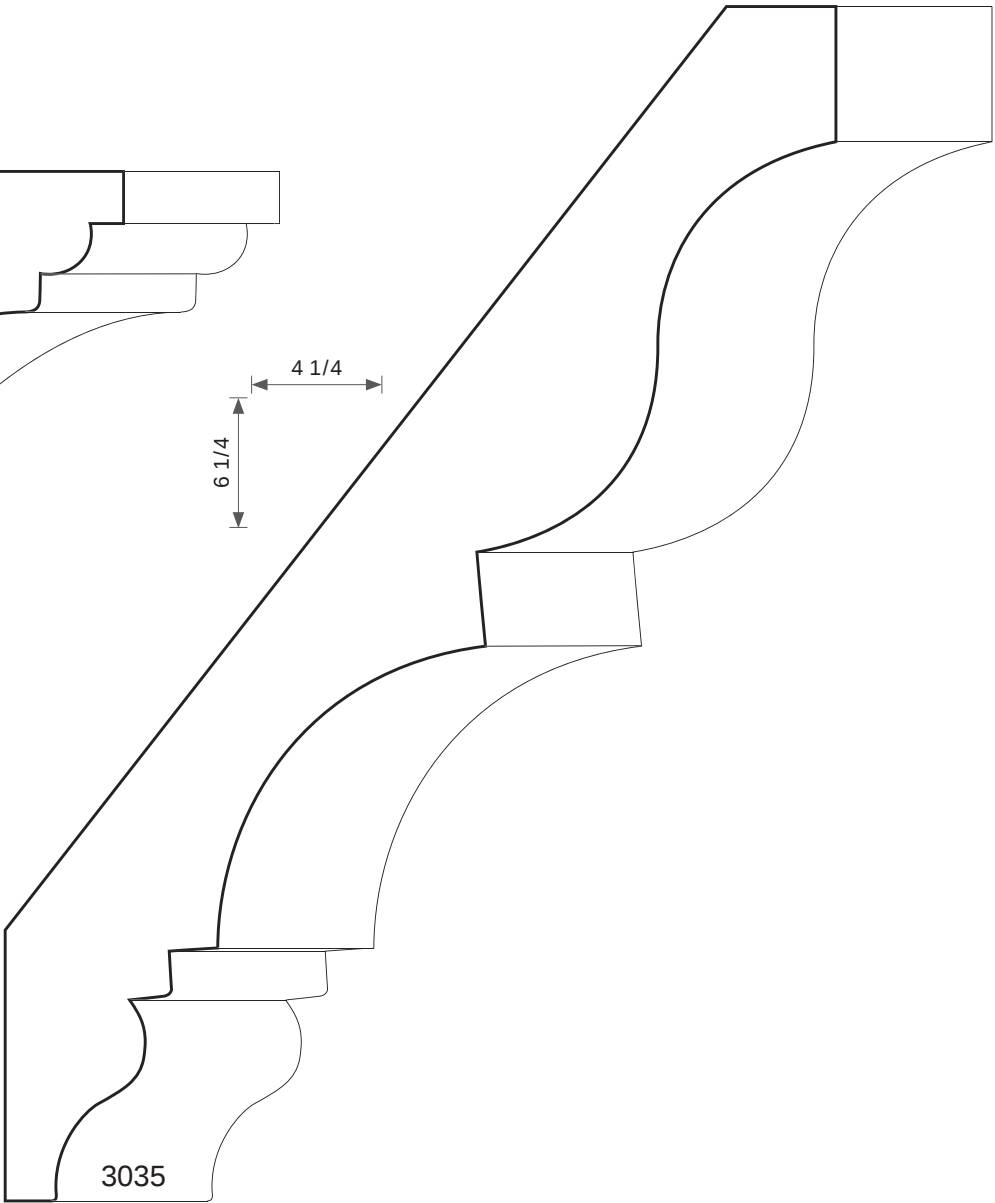
1-1/16T X 7-1/2W
