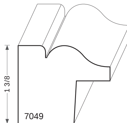
7049 RABBET 5/8 X 3/4
