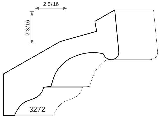
7/8T X 3-1/8W
