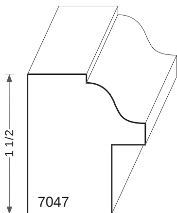
7047 RABBET 3/8 X 3/4
