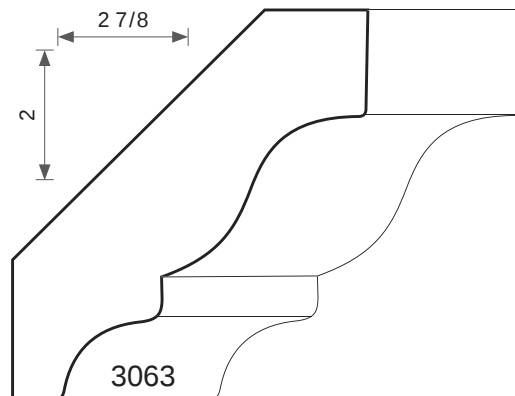
3/4T X 2-3/4W
