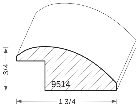
RABBET 1/2 X 1/2
